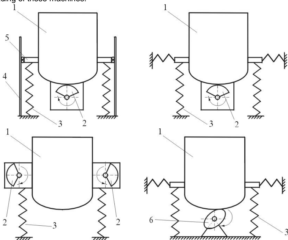
Fig. 1. Vibration technological machines for the implementation of compression of friable or tough moving loading or separation (mixing) of its
